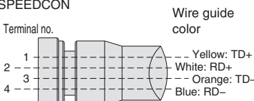
Plug connector pin arrangement D-coded
