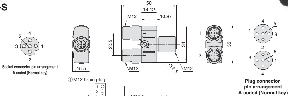
Solenoid valve power supply cable side pin arrangement when using a branch connector
